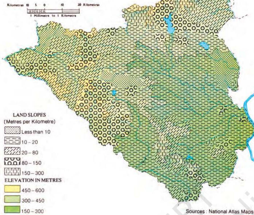
Figure 1.7 Relief and Slope Map of Nagpur District
