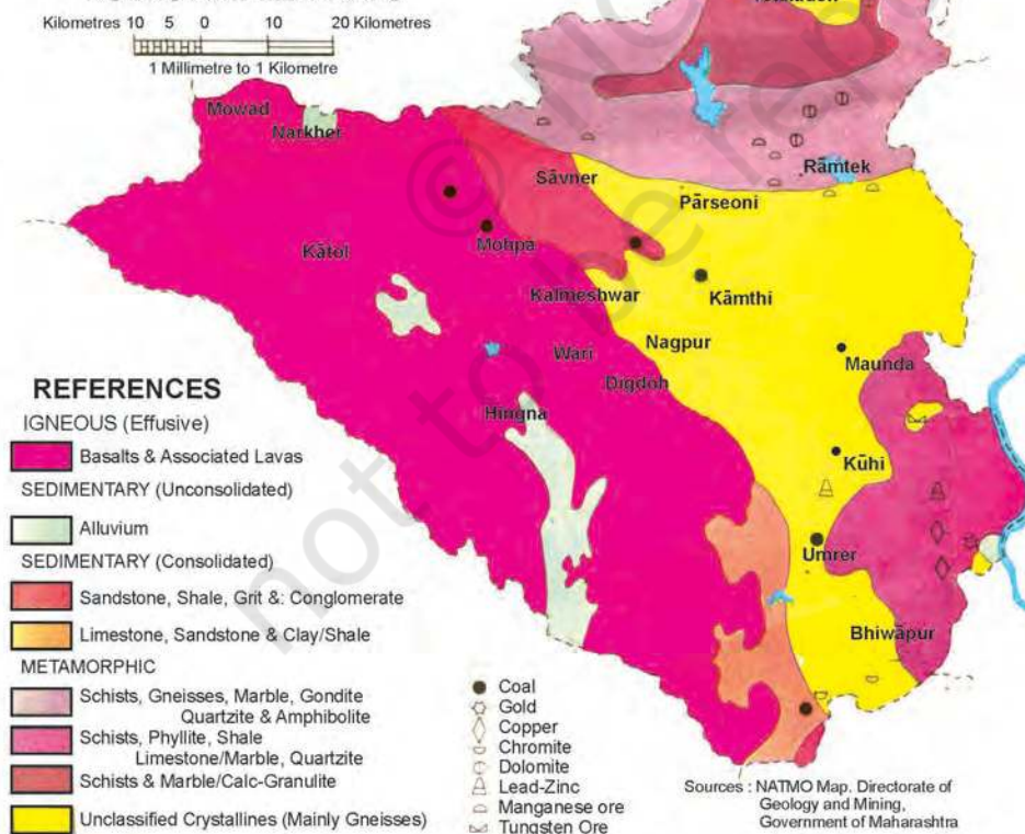
Figure 1.8 Distribution of Rocks and Minerals in Nagpur District
