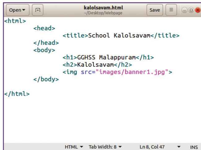
Fig. 8.6 Source of a web page in which an image is included
