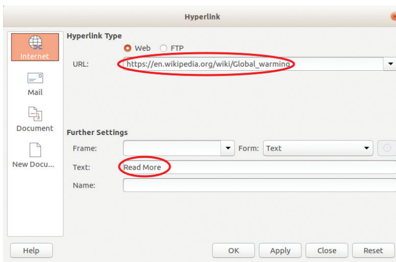
Fig.7.5 Hyperlink window
