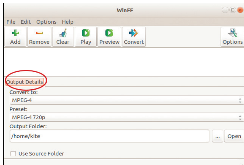
Fig. 9.11 WinFF window
