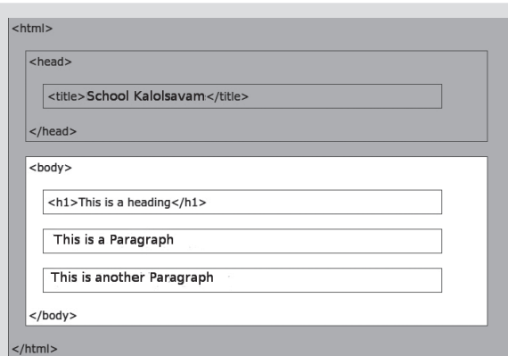
Fig. 8.1 HTML page layout
