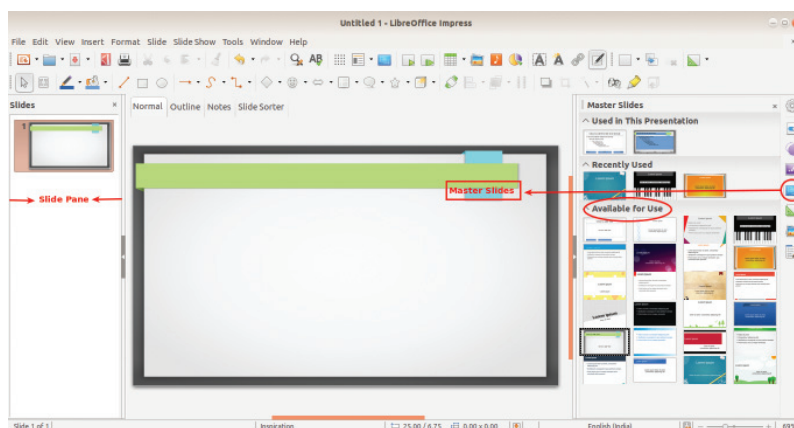
Fig. 7.1 Impress window
