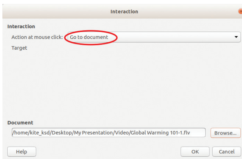
Fig.7.4 Interaction window
